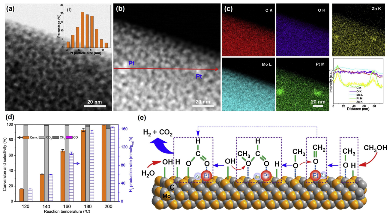
Fig. 7 (a) HRTEM image, (b) HAADF-STEM image, and (c) EDS element mapping and line spectra along the red arrow in (b) of 0.5% Zn-Pt/MoC. (d) Catalytic performance of 0.5% Zn-Pt/MoC for methanol steam reforming at different temperatures. (e) Proposed mechanism for methanol steam reforming on 0.5% Zn-Pt/MoC. 210 Modified with permission from ref. 210. Copyright (2020) Elsevier Inc.
