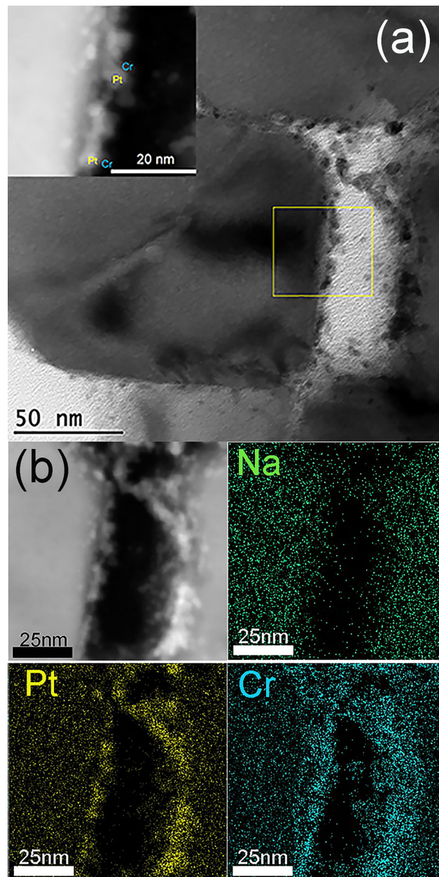
Fig. 7 (a) TEM and ADF-STEM (inset) images and (b) ADF-STEM image along with STEM-EDS elemental maps of the cross-section of a 0.9 wt% \text{Cr}_2\text{O}_3/0.23 \text{ wt% Na } 0.3 \text{ wt% Pt}/\text{BaTaO}_2\text{N:Zr0.01} sample.
