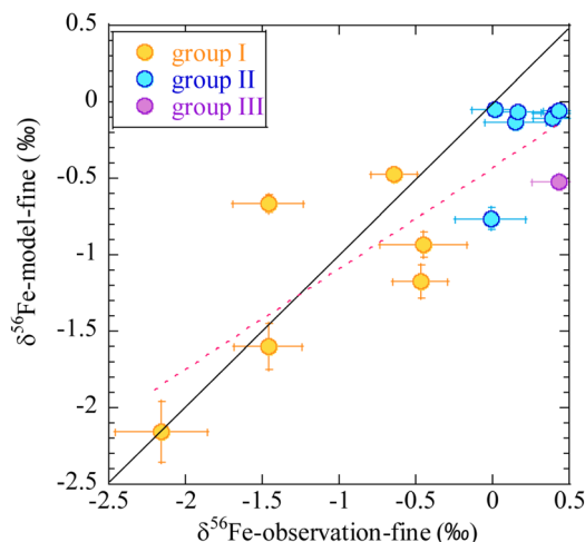
Fig. 8 Comparison of observed (horizontal axis) and numerical model estimates (vertical axis) of Fe stable isotope ratios in fine particles ( <2.5 \mu\text{m} ) over the western North Pacific. 137 The air masses are classified into three broad groups. The first group is mainly transported from the direction of East Asia. The second group is from the central and eastern Pacific. The third group is from the northern North Pacific. Adopted from ref. 137 under CC BY 4.0 with permission from Copernicus Publications, Copyright © The Author(s) 2021.
