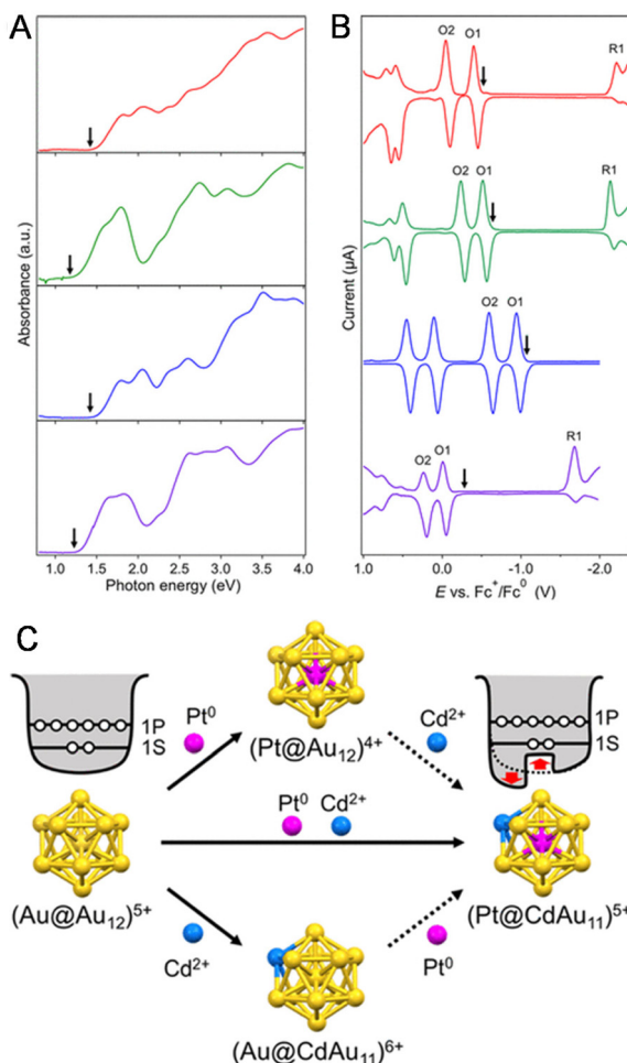
Fig. 14 (A) Ultraviolet–visible–near-infrared spectra and (B) DPV curves of [\text{Au}_{25}\text{PtCd}(\text{PET})_{18}]^{-} (red), [\text{Au}_{25}(\text{PET})_{18}]^{-} (green), [\text{Au}_{24}\text{Pt}(\text{PET})_{18}]^0 (blue), and [\text{Au}_{24}\text{Cd}(\text{PET})_{18}]^0 (purple) in benzene and \text{CH}_2\text{Cl}_2 , respectively. The downward arrows in panels (A) and (B) represent the corresponding optical H–L gaps and open-circuit potentials, respectively. (C) Schematic illustration of the jellium potentials of the (\text{Au}@\text{Au}_{12})^{5+} and (\text{Pt}@\text{CdAu}_{11})^{5+} superatoms. Reproduced with permission from ref. 116. Copyright 2020, American Chemical Society.
