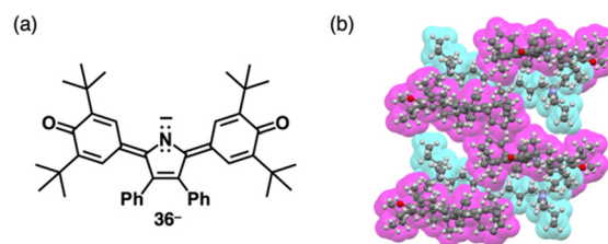
Fig. 22 (a) Deprotonated pyrrole-bridged quinone 36^- and (b) single-crystal X-ray structure of \text{TBA}^+-36^- (redrawn from a cif file: 2076443).
