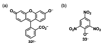
Fig. 20 (a) Uranine 32^{2-} and (b) deprotonated picric acid 33^- .
