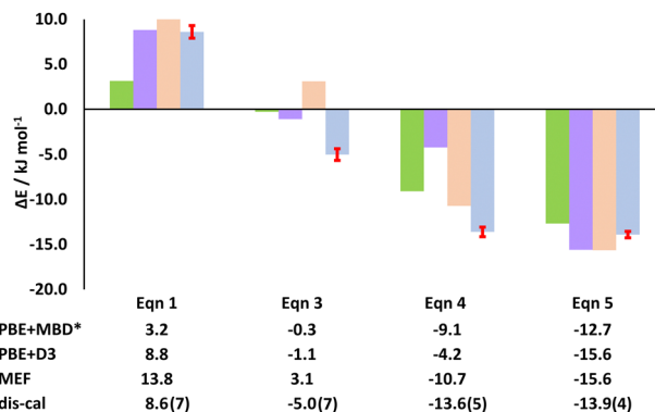
Fig. 2 Cocystal interconversion energies (in kJ mol -1 ) obtained from periodic DFT calculations, molecular energy frameworks (MEF) and dissolution calorimetry (dis-cal) measurements. Red error bars are shown for the energies measured by dis-cal.
