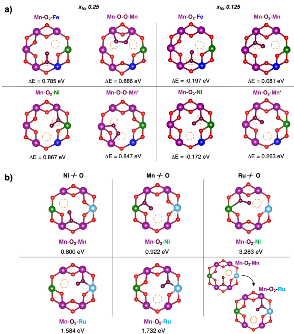
Fig. 6 Formation of dioxygen species in the Mn-deficient site of (a) Na_{1/4}Fe_{1/8}Ni_{1/8}Mn_{3/4-y}O_2 and (b) Na_{1/4}Ru_{1/8}Ni_{1/8}Mn_{3/4-y}O_2 . Corresponding formation energy, \Delta E , computed according to eqn (3) at PBE+ U (-D3BJ) are also reported. Colour code as in Fig. 5, O atoms at dioxygen positions are depicted in brown, Fe in blue and Ru in cyan. Reproduced from ref. 134 [A. Massaro et al., J. Am. Ceram. Soc. , 2023, 106 , 109–119]. Copyright ©2000–2022 by John Wiley & Sons, Inc. 134 Reproduced from ref. 135 [A. Massaro et al., ACS Appl. Energy Mater. , 2022, 5 (9), 10721–10730]. Copyright 2022 American Chemical Society. 135
