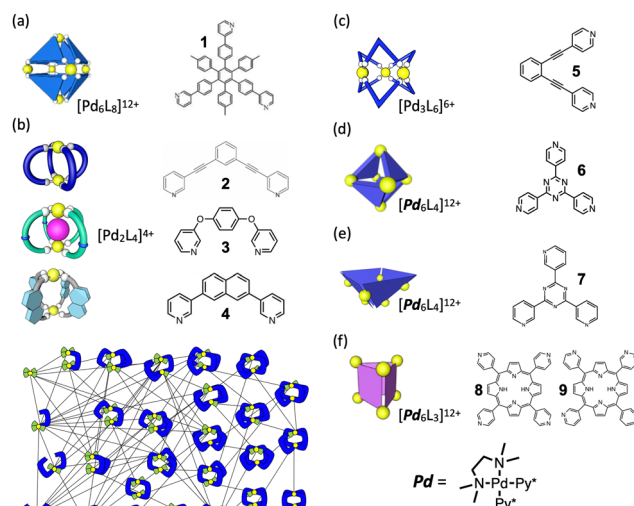
Fig. 2 Geometrical structures of the metal-organic coordination complexes whose self-assembly processes were investigated by NASAP so far. Multitopic ligand used to construct each self-assembly is also indicated. (a) [Pd_6L_8]^{12+} capsule. (b) [Pd_2L_4]^{4+} cages, for which the reaction network employed in the simulations is shown. (c) [Pd_3L_6]^{6+} double-walled triangle. (d) [Pd_6L_4]^{12+} truncated tetrahedron. (e) [Pd_6L_4]^{12+} square-based pyramid. (f) [Pd_6L_3]^{12+} prism. For (d)–(f) self-assemblies, the metal source Pd is cis -protected Pd(II) complex ( [Pd(TMEDA)]^{2+} ) where two coordination sites of the Pd(II) ion are occupied by a chelate ligand (TMEDA: N,N,N',N' -tetramethylethylenediamine).
