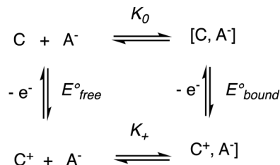
Scheme 11 Square scheme showing the association constant K_0 between the ferrocenyl dendrimer and the anion and that between the oxidized dendrimer and the anion ( K_+ ) as a function of the redox potentials of the ferrocenyl dendrimer alone before titration ( E_{\text{free}}^\circ ) and in the presence of the anion at the end of titration ( E_{\text{bound}}^\circ ). If K_0 is large (strong association of \text{A}^- with the ferrocenyl dendrimer), the second cyclovoltammetry wave appears during the titration. If K_0 is small (weak association), the unique wave progressively shifts during the titration upon addition of the anion salt.
