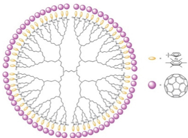
Fig. 9 Dendri-64[ \text{-NHC(O)-CpFe(II)}^+\text{C}_6\text{Me}_6\text{C}_{60}^{60+} ] (with Dendri = diamino-butane (DAB)-core G_5 dendrimer) from the reaction between Dendri-64[ \text{-NHC(O)-CpFe(II)}\text{C}_6\text{Me}_6 ] with 64 equiv. \text{C}_{60} . EPR: g = 2.00093 , \Delta H = 3.12 G. Reproduced with permission from ref. 74. Copyright 2012 Springer Nature.
