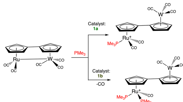
Scheme 2 ETC-catalyzed \text{PMe}_3 ligand addition in the fulvalene heterobimetallic complex [\text{RuW}(\eta^{10}\mu^2\text{-C}_{10}\text{H}_8)(\text{CO})_5] . The reaction depends on the \text{Fe(II/I)} redox potential of the electron-reservoir ETC catalyst ( 1a vs. [\text{Fe}(\eta^5\text{-C}_5\text{Me}_5)(\eta^6\text{-C}_6\text{Me}_6)] , 1b ). With the more electron-rich electron reservoir 1b as ETC catalyst, two \text{PMe}_3 ligands are introduced whereas, with 1a , only one \text{PMe}_3 ligand is added. ETC catalysis was pioneered by Henry Taube. 27
