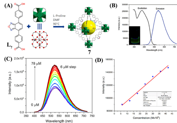
Fig. 4 (A) Synthesis of sensor LMOF 7 from ligand \text{L}_7 and \text{Zr(IV)} ; (B) Excitation and emission spectra of 7 were measured in \text{H}_2\text{O} (inset: photographs of 7 in \text{H}_2\text{O} ); (C) Changes in fluorescence emission intensity for 7 upon the gradual addition of aqueous \text{NH}_3 . (D) Linear fit for the \text{NH}_3 concentration–intensity correlation. Reprinted with permission from ref. 51. Copyright 2022 Royal Society of Chemistry.
