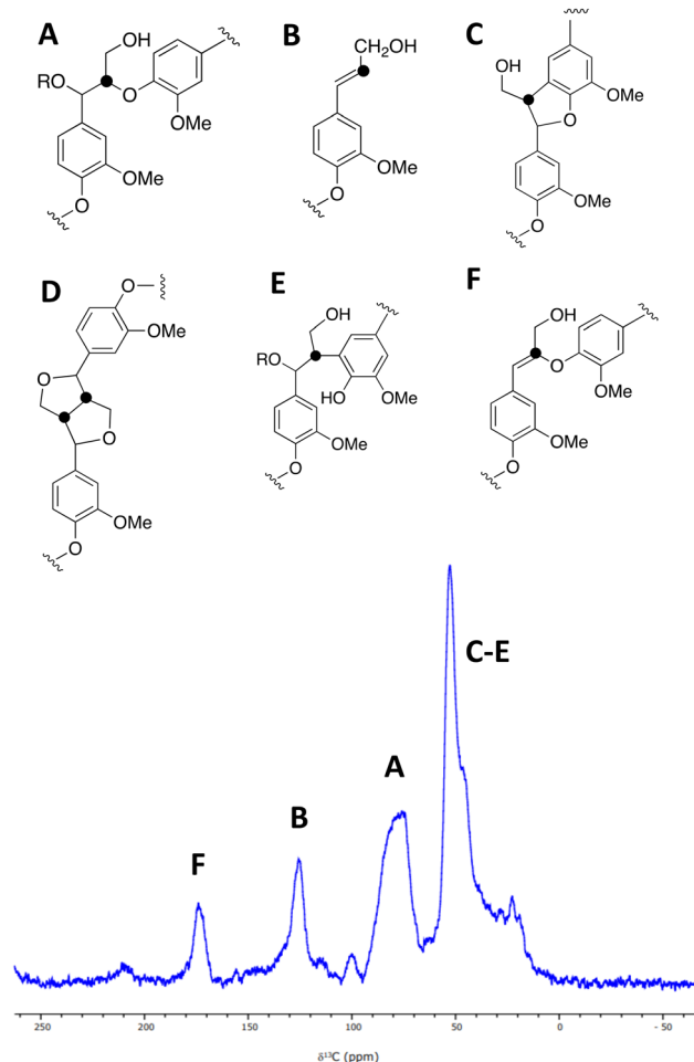
Fig. 3 A solid state 1 H (600 MHz)- 13 C CP (2 ms) MAS (12.5 kHz) NMR spectrum of [ \beta - 13 C]-labelled DHP lignin, and chemical structures of lignin substructures corresponding to the observed peaks. 10 240 transients were co-added for a recycle delay of 7 s.
