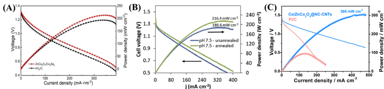
Fig. 18 Discharge polarization curves and the corresponding power density plots of a battery based on (A) ZnCo 2 O 4 /Co 3 Se 2 and IrO 2 /C (Reproduced with permission. 253 Copyright Marketplace™. Royal Society of Chemistry), (B) annealed and unannealed W-Co oxide electrodes (Reproduced with permission. 252 Copyright © 2020 Hydrogen Energy Publications LLC. Published by Elsevier Ltd. All rights reserved) and (C) Pt/C and Co/ZnCo 2 O 4 @NC-CNTs (Reproduced with permission. 255 Copyright © 2020 Elsevier Ltd. All rights reserved).
