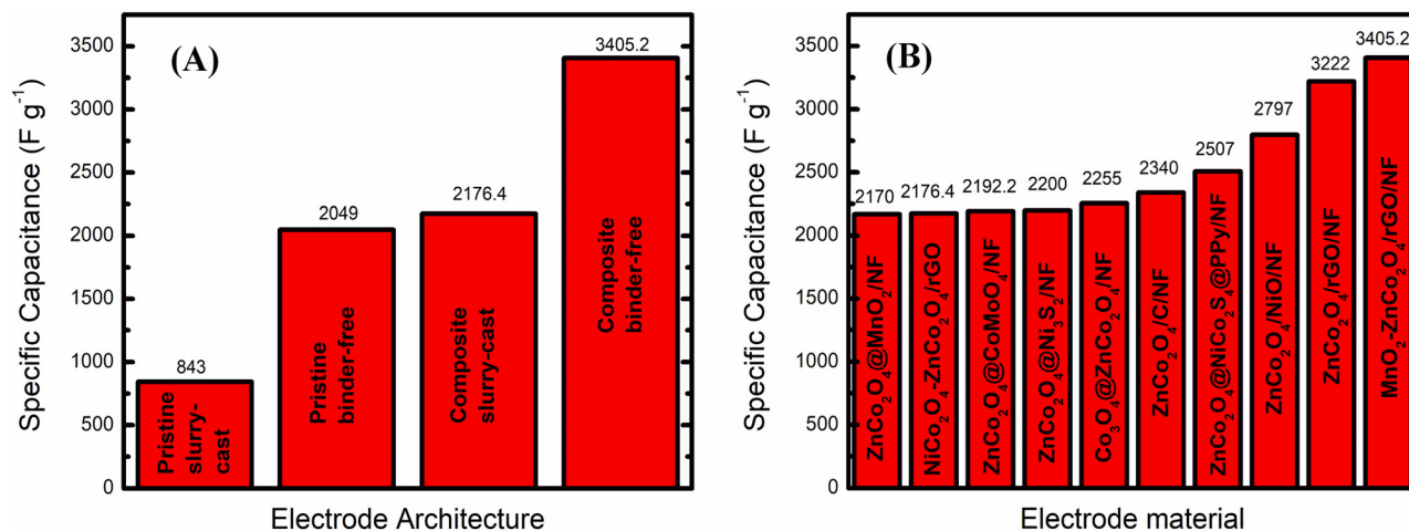
Fig. 13 (A) Best specific capacitance for each \text{ZnCo}_2\text{O}_4 -based electrode type: pristine slurry-cast; pristine binder-free; composite slurry-cast and composite binder-free (ref. 11, 26, 58 and 62, respectively). (B) Top 10 specific capacitances delivered by \text{ZnCo}_2\text{O}_4 -based electrodes (ref. 62, 43, 38, 90, 84, 67, 75, 79, 58 and 89, respectively).
