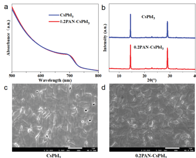
Fig. 1 UV-vis (a) and XRD (b) spectra of CsPbI 3 and 0.2PAN–CsPbI 3 thin films, and top-surface SEM images of CsPbI 3 (c) and 0.2PAN–CsPbI 3 films (d). Scale bar, 1 \mu m.
