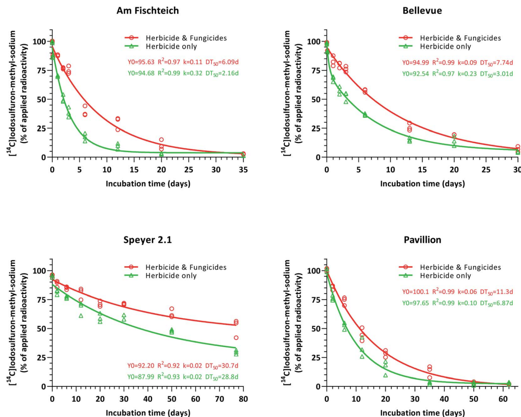
Fig. 4 Recovery (in %AR) of [ ^{14}\text{C} ]-iodosulfuron-methyl-sodium from soil samples ( n = 3 ). Triangular data in green depict soil samples treated with iodosulfuron-methyl-sodium only (controls), circular data in red describe soil samples treated with tebuconazole and prothioconazole 14 days prior to (day -14; dose 1), then on the same day as the herbicide treatment (day 0; dose 2), and again 5 days after application of radiolabeled iodosulfuron-methyl-sodium (day 5; dose 3).
