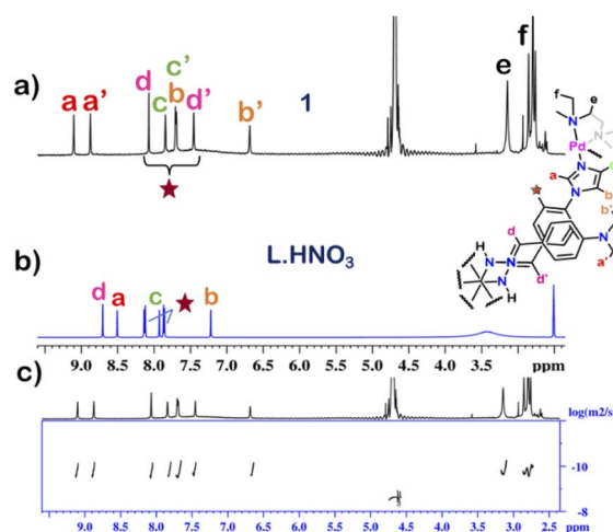
Fig. 1 Stacked 1 H NMR spectra of the (a) cage 1 in D 2 O, (b) ligand L \cdot HNO_3 in DMSO- d_6 and (c) diffusion-ordered 1 H NMR of 1 in D 2 O.
