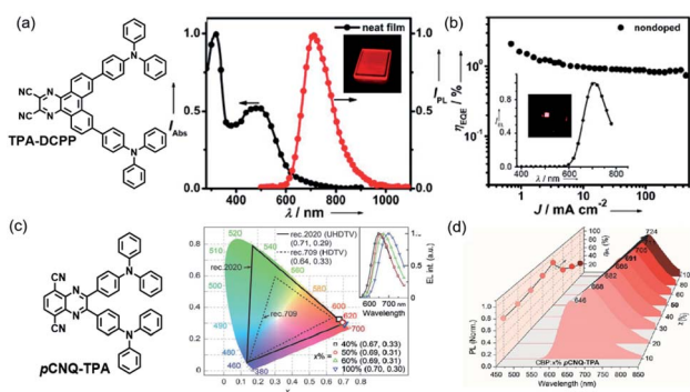
Fig. 2 (a) The absorption (black) and PL (red) spectra of TPA-DCPP in a neat film. Inset: image of the neat film under UV irradiation ( \lambda_{\text{ex}} = 365 \text{ nm} ). Copyright 2015, John Wiley & Sons. (b) EQE versus current density characteristics of the TPA-DCPP based non-doped device. Inset: EL spectrum and image of the device at 5 V. Copyright 2015, John Wiley & Sons. (c) Coordinates of the devices in CIE space and corresponding EL spectra (insets). Copyright 2021, John Wiley & Sons. (d) Variations of photoluminescence (PL) spectra and PL quantum yields for CBP: x % p CNQ-TPA films ( x = 10–100). Copyright 2021, John Wiley & Sons.
