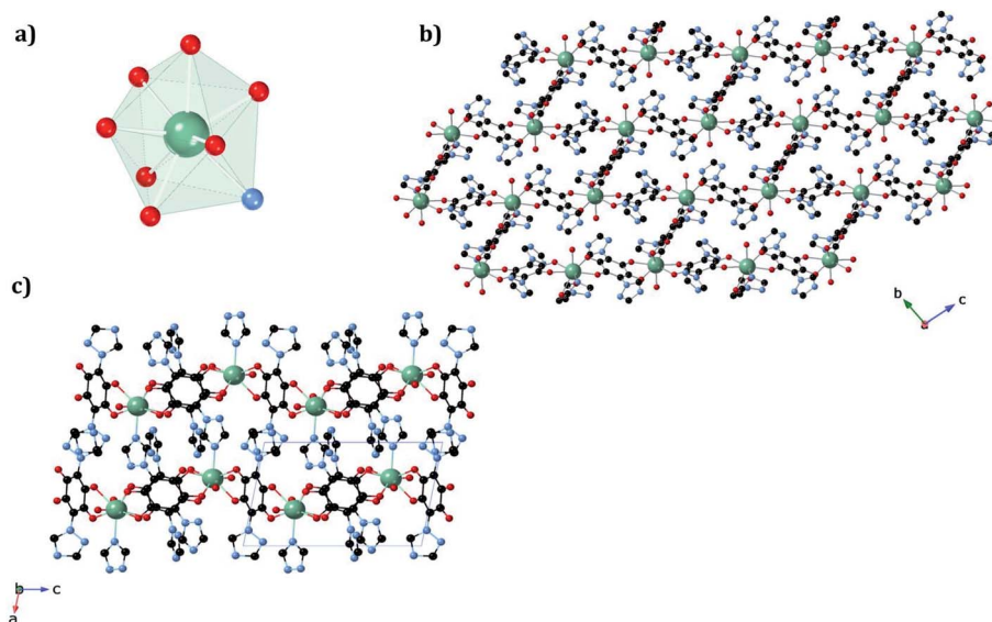
Fig. 4 (a) Triangular dodecahedron coordination geometry of the \text{Er}^{\text{III}} ions in 1a des . (b) View along the bc plane of the 1a des framework, showing shrunken rectangular cavities. (c) View along the ac plane of 1a des , showing layers bridged by \text{trz}_2\text{An} linkers. The black, blue, red, and green spheres represent the C, N, O, and \text{Er}^{\text{III}} atoms, respectively. Hydrogen atoms and water molecules inside the pores are omitted for clarity.
