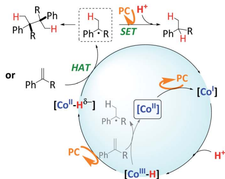
Scheme 5 Possible mechanistic scenarios for the reduction of aromatic olefins by the light-driven dual-copper–cobalt catalytic system in aqueous media. The highlighted [Co II ] intermediate indicates the beginning of the catalytic cycle. Acronyms stand for PC = photoredox catalyst; ED = electron donor; SET = single electron transfer and HAT = hydrogen atom transfer.
