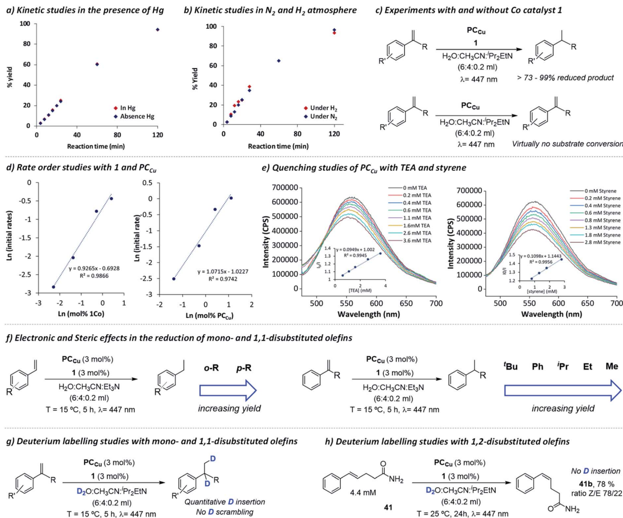
Fig. 1 Mechanistic studies. Formation of 16a in (a) the absence (red diamonds) and presence of Hg(0) (>2000 eq.) (blue diamonds); and in (b) \text{H}_2 (red diamonds) or \text{N}_2 (blue diamonds) atmosphere. (c) Experiments with and without complex 1 . (d) Reaction rate kinetics regarding complex 1 and \text{PCu} . (e) Reductive quenching studies of \text{PCu} with TEA and styrene. (f) Steric effects in alkene reduction. Deuterium labelling studies of mono- and 1,1-disubstituted olefins (g) and 1,2-disubstituted olefin 41 (h, Z/E ratio analysed by NMR). See Experimental section 3 for the procedure details.†
