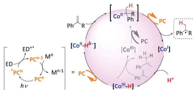
Scheme 5 Possible mechanistic scenarios for the reduction of aromatic olefins by the light-driven dual-copper–cobalt catalytic system in aqueous media. The highlighted [Co II ] intermediate indicates the beginning of the catalytic cycle. Acronyms stand for PC = photoredox catalyst; ED = electron donor; SET = single electron transfer and HAT = hydrogen atom transfer.
