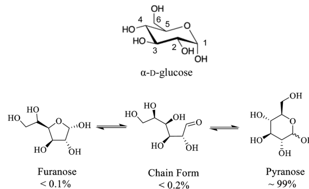
Scheme 1 (Top) Molecular structure of \alpha\text{-D-glucose} where carbon atoms are numbered. (Bottom) different \text{D} -glucose tautomers present in aqueous solution.
