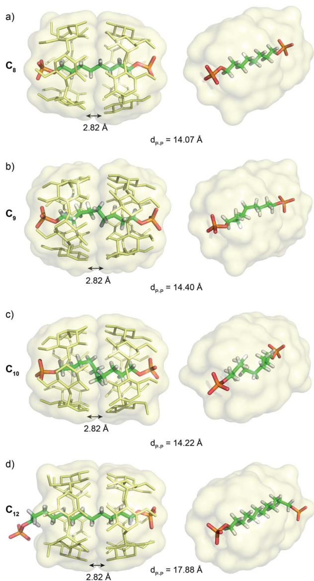
Fig. 4 Crystallographic structures of [3]pseudorotaxanes with (a) C 8 , (b) C 9 , (c) C 10 and (d) C 12 axles showing 5 gauche conformations for the C 10 axle resulting in a compression of the alkyl chain. Hydrogen atoms, except on the axle, and counter anions have been omitted for clarity.
