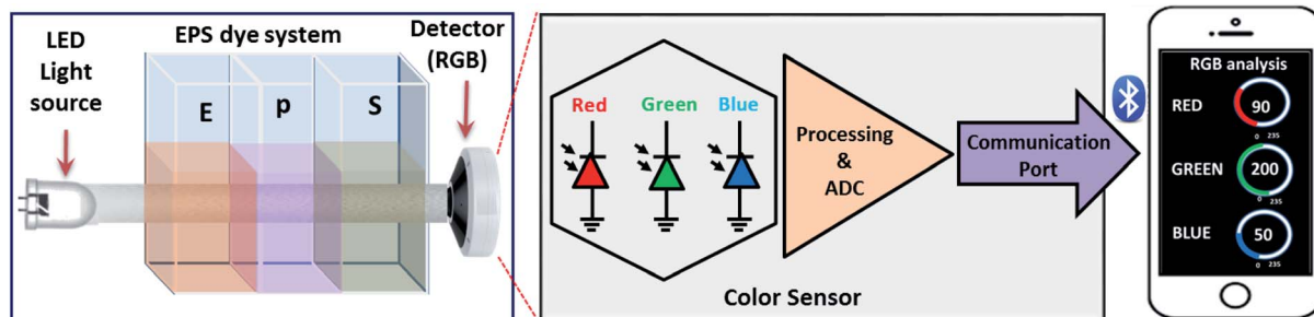
Fig. 1 Fabricated smartphone-assisted sensor prototype.
