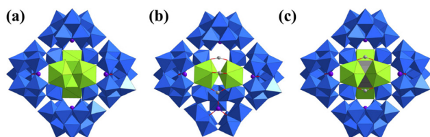
Fig. 12 Views of (a) [U_2(\mu_2-OH)_3(\mu_2-O)\{As_4W_{40}O_{140}\}]^{25-} , (b) [U_2(\mu_2-O)(HCOO)_3\{As_4W_{40}O_{140}\}]^{25-} , and (c) [U_4(\mu_2-O)_2(HCOO)_4\{As_4W_{40}O_{140}\}]^{20-} . Color codes are the same as in Fig. 1.
