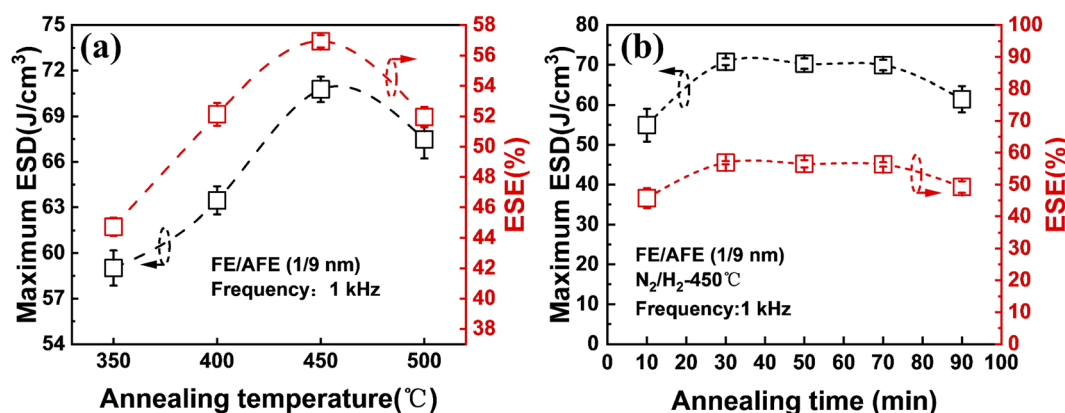
Fig. 3 The maximum ESD and corresponding ESE of the capacitor with the FE (1 nm)/AFE (9 nm) stack: (a) at different annealing temperatures for 30 min; (b) at 450 \text{ } ^\circ\text{C} for different annealing times. Ten devices are measured for each sample.
