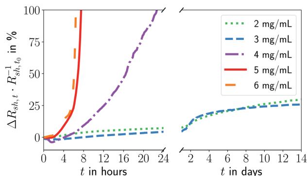
Fig. 1 Relative change in sheet resistance ( R_{sh,t} - R_{sh,t_0} )/ R_{sh,t_0}^{-1} = \Delta R_{sh,t} \cdot R_{sh,t_0}^{-1} after time t for electrodes imprinted at different ink concentrations c_{Au} . The results of repeated experiments and additional concentrations are shown in Fig. S1 in the ESI†
