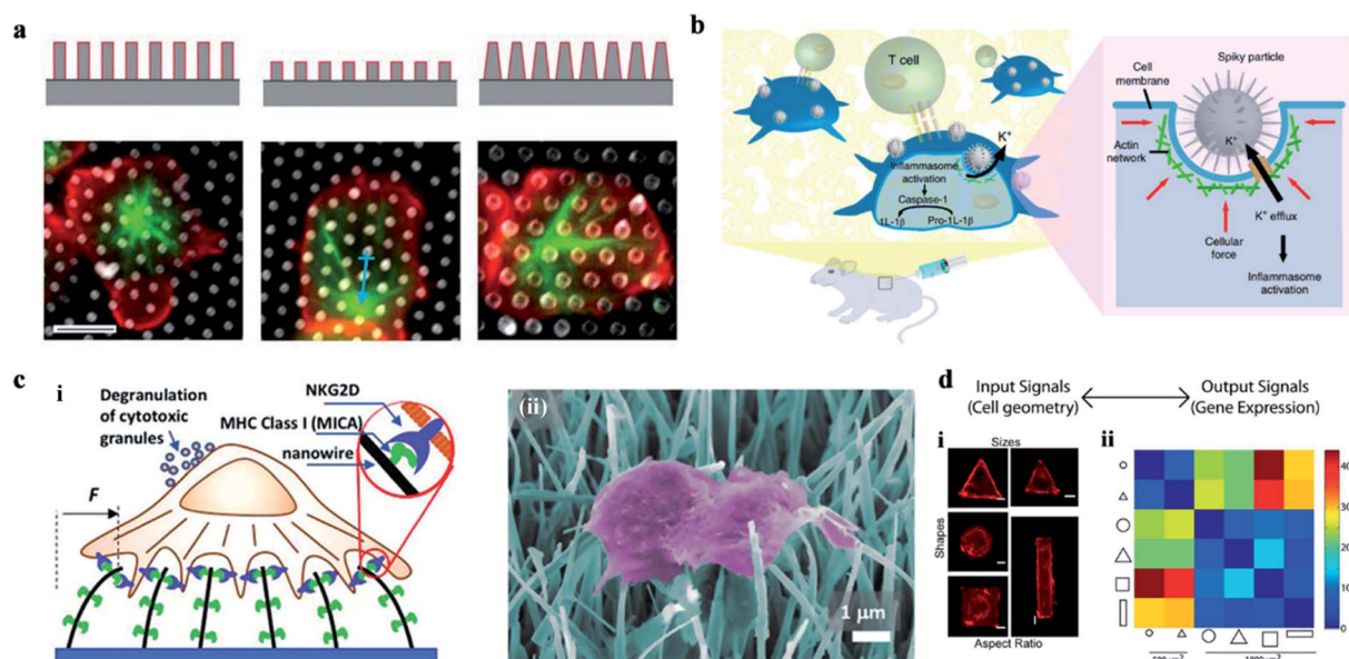
Fig. 8 (a) The effect of a 3-D structure on T cell activation. Images illustrate the microtubule structure (green, \beta -tubulin) and cell morphology (red, CD45). Scale bar, 5 \mu m . 126 (b) Schematic of spiky particles applied to activate immune cells and amplify immune responses in vivo . 74 (c) (i) Schematic drawing of NK activation on MICA-functionalized nanowires. (ii) SEM image of NK cells on MICA-functionalized nanowires. 132 (d) Cell geometry imposes modular changes in gene expression. (i) NIH 3T3 fibroblast cells cultured on fibronectin coated patterns of different sizes, shapes, or AR (AR is defined as cell adhering to micropatterns of similar area but different ratios of short axis to long axis.) (ii) Two-dimensional matrix showing the total number of differentially regulated genes among cells of different geometries. 134 Reprinted with permission Copyright 2019, PNAS; Nature Nanotechnology 2018; Advance Materials 2019; 2013, PNAS.
