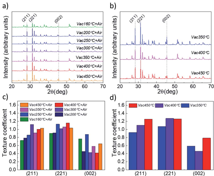
Fig. 6 XRD patterns of CSS \text{Sb}_2\text{Se}_3 absorber films deposited at 460 °C onto \text{TiO}_2/\text{FTO}/\text{glass} stacked substrates, with (a) vacuum and subsequent air annealed (Vac+Air) \text{TiO}_2 and (b) vacuum annealed only (Vac) \text{TiO}_2 layers. Related texture coefficients (TC) for (c) vacuum and subsequent air annealed (Vac+Air) and (d) vacuum annealed (Vac) films, calculated from the integrated intensity ratios (using the Harris formula 46 ) for the dominant miller planes of \text{Sb}_2\text{Se}_3 .
