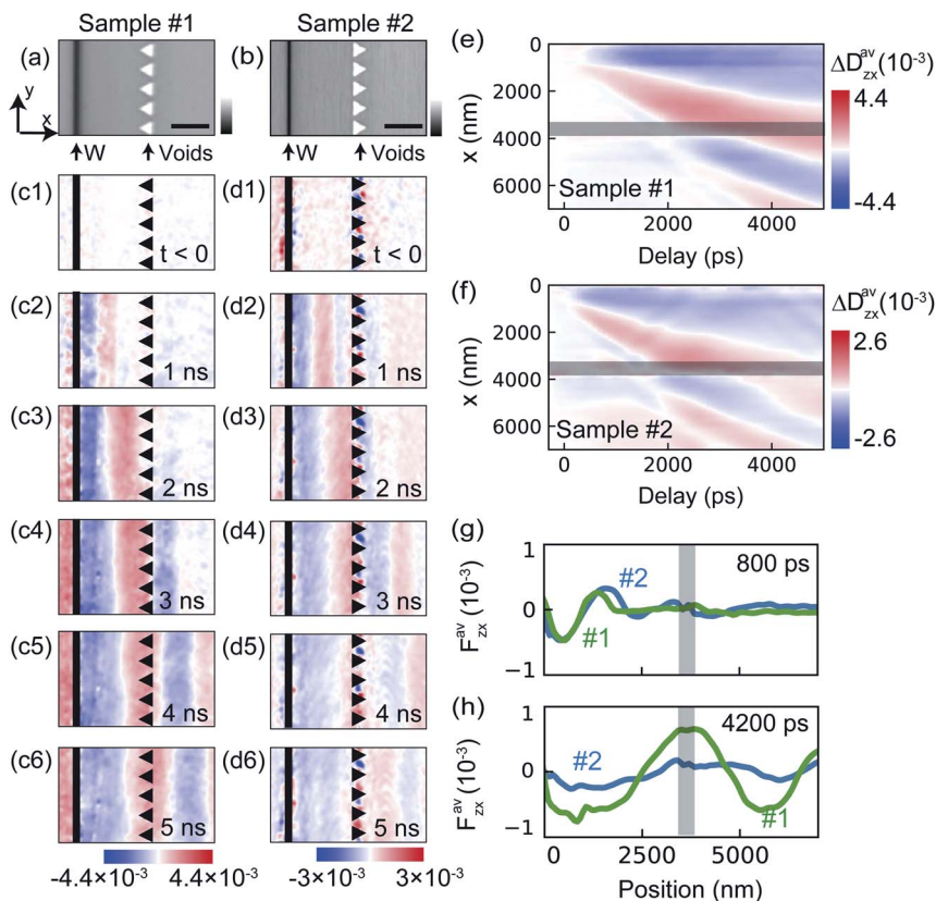
Fig. 5 (a and b) Bright-field images of Samples #1 and #2. The scale bar denotes 2 μm. The black region corresponds to the deposited tungsten bar. The white triangles are voids fabricated by FIB. (c and d) Time dependence of \Delta D_{zx}(x,y,t) calculated by the 5D-STEM-CBED analysis. The black line and triangles indicate the deposited tungsten bars and the triangular voids, respectively. (e and f) Position and time dependence of \Delta D_{zx}^{av}(x,t) for Samples #1 and #2, obtained by averaging \Delta D_{zx}(x,y,t) along the y direction. (g and h) \Delta D_{zx}^{av}(x,t) at 800 and 4200 ps, respectively. The gray shaded regions in (e-h) denote the position where the triangular void patterns are fabricated.
