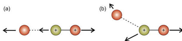
Fig. 10 Proposed dissociation mechanism of \text{SO}_2 at an electron energy of 100 eV for the ( \text{S}^+, \text{O}^+ ) covariance channel. The red atoms correspond to oxygen, and the green-yellow atoms to sulfur. (a) Shows the case where the \text{SO}_2^{2+} dication is linear. In this case, the departing \text{S}^+ ion is hindered by the presence of the neutral O atom, leading to a smaller kinetic energy than might otherwise have been the case. (b) Shows a case where the \text{SO}_2^{2+} dication is bent. The kinetic energy of the \text{S}^+ ion is greater than in case (a), but the trajectory is deflected due to the presence of the neutral O.
