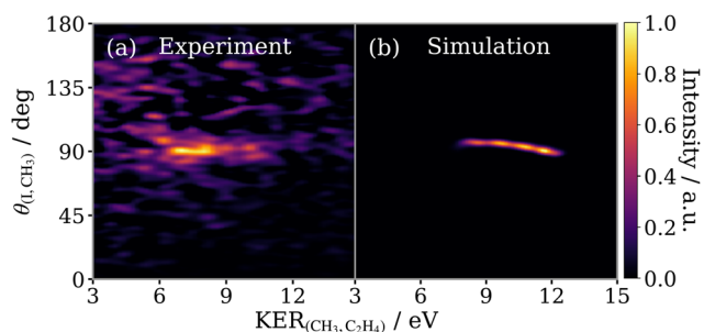
Fig. 8 Experimental (a) and simulated (b) covariance maps for concerted three-body breakup of 2\text{-IP}^{3+} as a function of KER of the secondary products ( \text{KER}_{\text{CH}_3, \text{C}_2\text{H}_4} ) and the relative recoil angle between the iodine and methyl ions ( \theta_{\text{I}, \text{CH}_3} ). Each panel is normalised separately.
