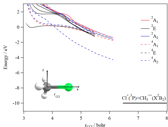
Fig. 9 spd(f) cc-pV5Z MRCI one-dimensional cuts of the PESs of the doublet and quartet states of \text{CH}_3\text{Cl}^{3+} by lengthening the CCl distance ( r_{\text{CCl}} ) (top) and by lengthening the CH distance ( r_{\text{CH}} ) (bottom). The remaining coordinates were set to their equilibrium values in \text{CH}_3\text{Cl} ( X^1A_1 ). These curves are given relative to the energy of the lowest \text{CH}_3\text{Cl}^{3+} doublet state at the \text{CH}_3\text{Cl} ( X^1A_1 ) equilibrium.
