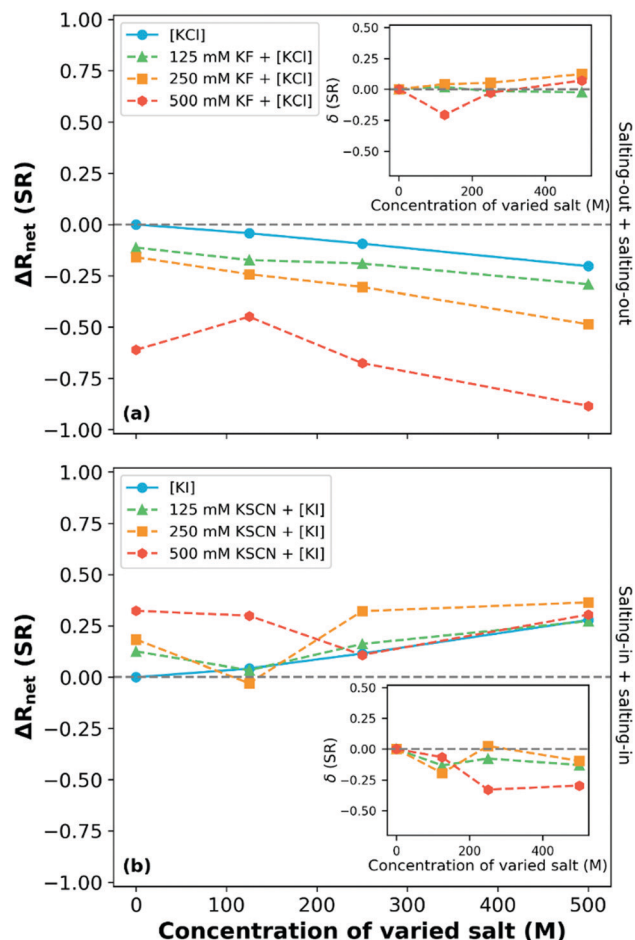
Fig. 14 The net response ( \Delta R_{\text{net}}(\text{SR}) ; change in swelling ratio relative to the response in water) of a \text{P}(\text{MEO}_2\text{MA}-\text{stat}-\text{OEGMA}_{300}) 80:20 mol% copolymer brush at 15 °C in binary electrolytes composed of (a) salting-out and (b) salting-in ions where the varied species is denoted by square brackets. Inset plots present the \delta values for the various binary electrolyte compositions. Adapted from ref. 249 with permission from Elsevier, copyright 2021.
