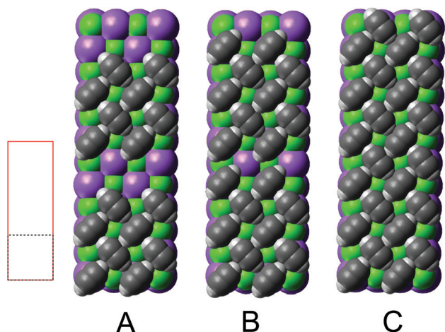
Fig. 3 Structure models A, B, and C for the system \text{NaCl}(100)/(\sqrt{3}\sqrt{2} \times \sqrt{2})R45^\circ\text{-C}_2\text{H}_2 with 4, 5, and 6 translationally inequivalent molecules per unit cell, respectively. Shown are 2 \times 2 unit cells in top view. The red square rectangle on the left illustrates the extension of the surface unit cell, while the dashed line indicates the reduced size of a (\sqrt{2} \times \sqrt{2})R45^\circ cell. See also Table 1.
