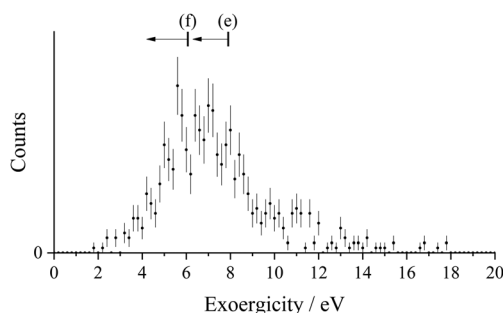
Fig. 4 Experimental exoergicity spectrum for the reaction \text{S}^{2+} + \text{H}_2 \rightarrow \text{S}^+ + \text{H}_2^+ . The error bars represent two standard deviations of the associated counts. The NDSET pathways indicated ((e) and (f)) are discussed in the text and the arrows on the labels indicate the direction of the expected broadening upon population of excited vibrational states of \text{H}_2^+ .
