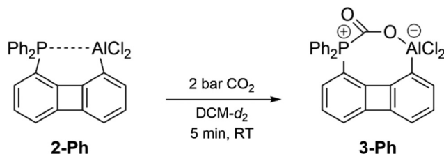
Scheme 3 Activation of CO 2 by 2-Ph .
