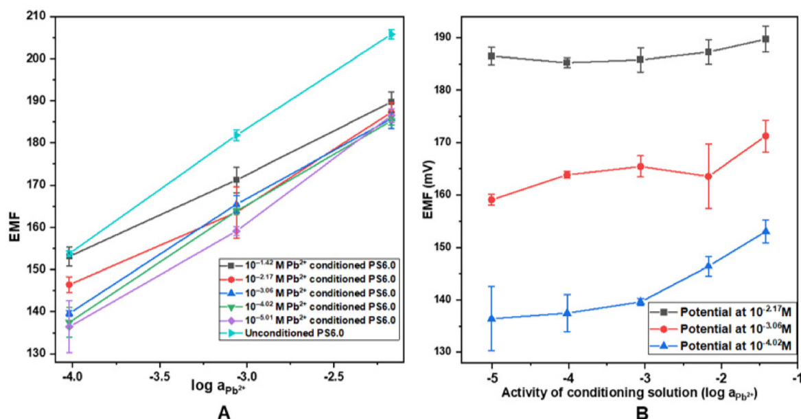
Fig. 4 Potentiometric response of Pb^{2+} -ISEs coupled with PS6.0 treated with different concentrations of Pb^{2+} (A) and variation of EMF at different Pb^{2+} activities for Pb^{2+} -ISEs coupled with ISM component modified paper substrates conditioned with different activities of Pb^{2+} (B).
