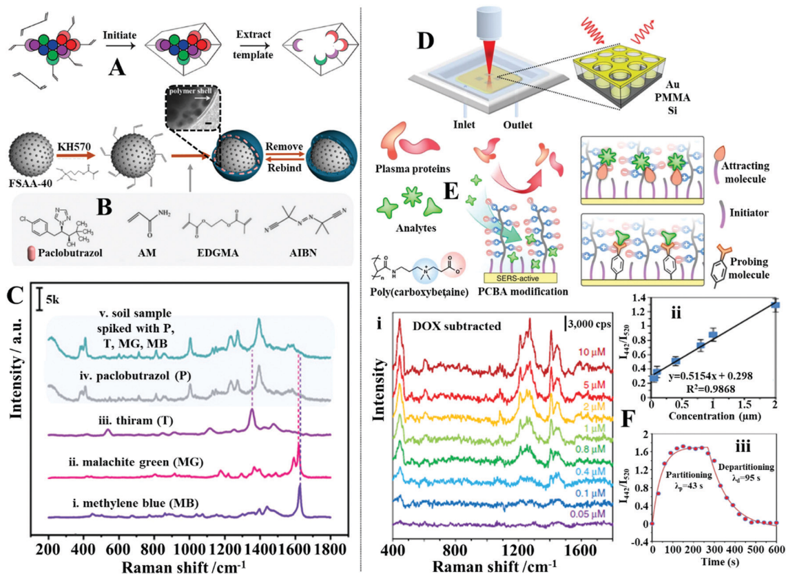
Fig. 12 (A) Schematic illustrations of the working principles of molecularly imprinted polymers (MIPs); (B) schematic illustration of the preparation of Fe 3 O 4 @SiO 2 -Au@Ag (FSAA) MIPs. Inset shows a TEM image of the product FSAA MIPs; (C) SERS spectra set demonstrating the selectivity of the FSAA MIP sensors. Spectra (i–iv) correspond to the SERS signals of the target analyte paclobutrazol and three contaminants, namely, thiram, malachite green and methylene blue. Spectrum v corresponds to the SERS signals obtained from a soil sample spiked with all four chemicals; (D) schematic illustrations of the SERS optofluidic system; (E) schematic illustrations of the different types of mixed self-assembled monolayers functionalized on the surface of the enhancing material to achieve anti-fouling and target recognition; (F) panel (i) show SERS spectra of Doxorubicin in plasma ultrafiltrate control at concentrations ranging from 0.05 to 10 μM. The background signals from plasma have been subtracted. Panel (ii) shows the linear region of the Doxorubicin detection curve generated by plotting the average intensity ratio of the doxorubicin peak at 442 cm -1 and plasma peak at 520 cm -1 as a function of doxorubicin concentration. The error bars stand for standard deviations obtained from three replicates. Panel (iii) shows partitioning and departitioning kinetics of 20 mM Doxorubicin in plasma on the anti-fouling SERS sensor. Panel (A) reproduced with permission from ref. 178, copyright 2017 American Chemical Society. Panel (B and C) adapted with permission from ref. 75, copyright 2020 American Chemical Society. Panel (D–F) adapted with permission from ref. 182, copyright Springer Nature Limited.
