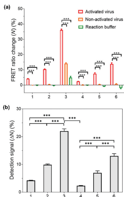
Fig. 5 Influenza virus detection with PNPs. (a) FRET ratio changes ( N ) after incubation with H9N2 viruses ( 10^{3.833} TCID 50 /mL). Each PNP was incubated with activated viruses in the presence of trypsin and acidic buffer (red), with non-activated viruses in the absence of trypsin and acidic buffer (orange), and in a solution containing trypsin and acidic reaction buffer (green). (b) Detection signals obtained from the PNPs with H9N2 viruses. The average detection signals ( \Delta N ) were obtained by subtracting FRET ratio changes ( N ) of the activated groups from non-activated virus groups. Samples are: 1: PNP (1k, 0.3), 2: PNP (1k, 0.45), 3: PNP (1k, 0.6), 4: PNP (2k, 0.3), 5: PNP (2k, 0.45), and 6: PNP (2k, 0.6). Box plots represent mean \pm standard deviation ( n = 3 ). Student's t -test was used for statistical analysis of the measured FRET ratio changes and detection signals between the groups (***) p < 0.0001 .
