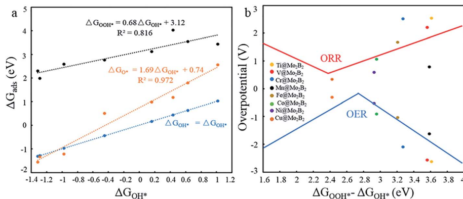
Fig. 6 (a) Scaling relationship between the \Delta G_{\text{OH}^*} and \Delta G_{\text{O}^*} , \Delta G_{\text{OOH}^*} at site I. (b) Dual volcano plot for the OER and ORR for TM@ \text{Mo}_2\text{B}_2 at site I.
