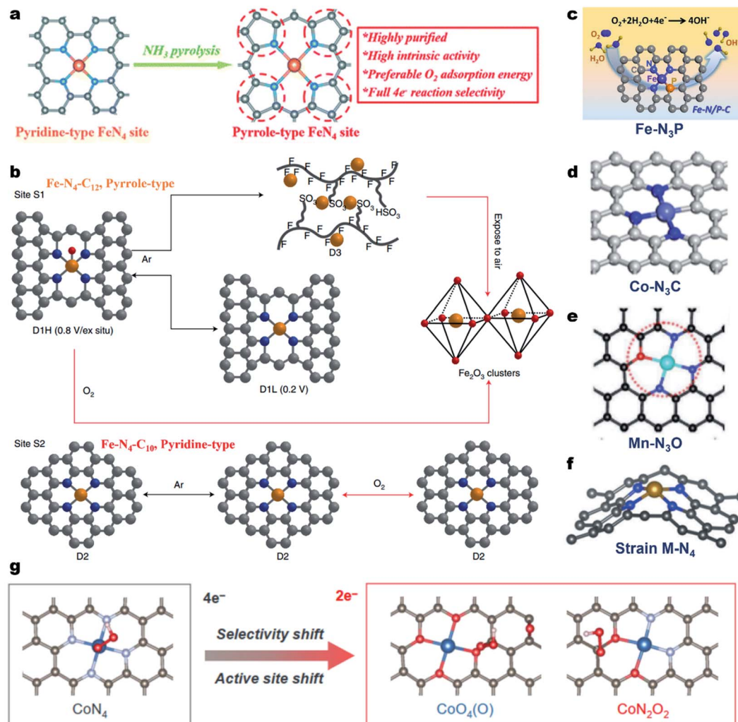
Fig. 2 Regulation of the coordination geometry of the metal center for enhancing the ORR activity. (a) Preparation process of the high-purity pyrrole-type Fe- \text{N}_4 structure. Reproduced with permission from ref. 97. Copyright (2020) Royal Society of Chemistry. (b) Coordination and structural changes of the sites S1 and S2 under in situ or operando conditions. Reproduced with permission from ref. 98. Copyright (2020) Springer Nature. (c) Schematic showing the N and P co-ordinated single Fe site (Fe- \text{N}_3\text{P} ). Reproduced with permission from ref. 104. Copyright (2020) American Chemical Society. (d) Schematic showing the N and C co-ordinated single Co site (Co- \text{N}_3\text{C} ). Reproduced with permission from ref. 106. Copyright (2020) American Chemical Society. (e) Schematic showing the N and O co-ordinated single Mn site (Mn- \text{N}_3\text{O} ). Reproduced with permission from ref. 109. Copyright (2018) Wiley-VCH. (f) Schematic showing the strained M- \text{N}_4 site. Reproduced with permission from ref. 112. Copyright (2019) WILEY-VCH. (g) \text{OOH}^* adsorption on \text{CoN}_4 and \text{CoO}_4(\text{O}) , and \text{CoN}_2\text{O}_2 sites. Reproduced with permission from ref. 117. Copyright (2021) American Chemical Society.
