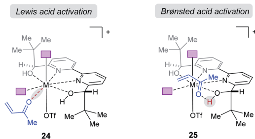
Fig. 7 (A) Enantiomers arise from enolate conformation and substrate facial approach. (B) Illustration of the relevant catalytic modes of activation for protonated ligands. Purple boxes denote enolate substrate.
