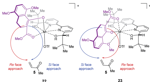
A. Possible metal-enolate binding conformations and ketone approaches
