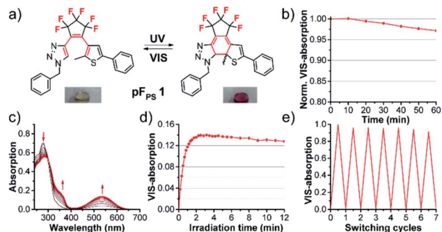
Fig. 3 Photochromism of pFps 1 (60 \mu M solution in \text{CHCl}_3 , irradiation at 310 nm, LED): (a) reversible electrocyclic ring closure, insets: photo of vial with colored solution, (b) thermostability of the closed form, monitored for 1 h at 20 ^\circ\text{C} at the VIS absorption maximum (534 nm), (c) evolution of the absorption spectra upon UV irradiation from the open form (black) towards the (pseudo-)photostationary state (p)PSS (red), (d) kinetic trace of the absorbance at 534 nm (VIS absorption maximum of the closed isomer) during prolonged UV irradiation, (e) reversibility measurement by alternating 310 nm and white-light illumination.
