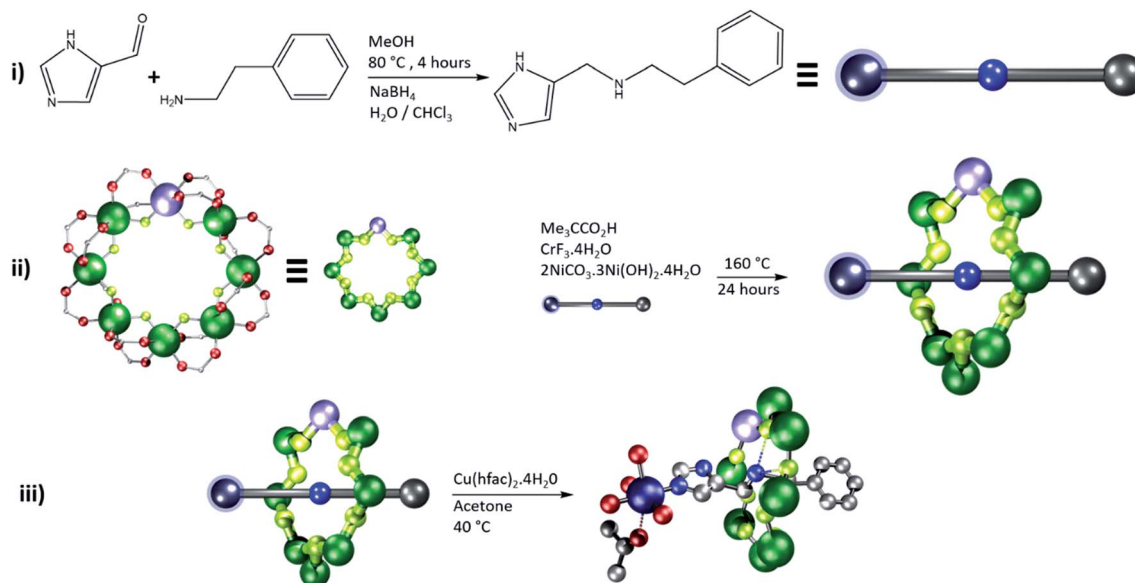
Fig. 2 Schematic diagram to show synthesis of compounds 2 , 4 , 8 and 10 . Showing 2 as a specific example. (i) Reductive amination to form the precursor thread. (ii) Synthesis of the ring around the thread to form a [2]rotaxane. (iii) binding the \text{Cu}^{\text{II}} ion and crystallization of the product. Atom colors: blue (N), red (O), grey (C), green (Cr), lilac (Ni), navy (Cu), yellow (F).
