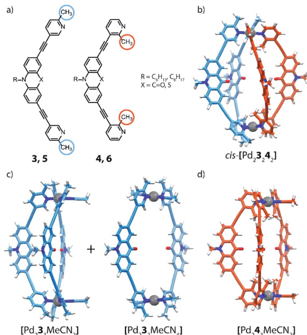
Fig. 5 (a) Banana-shaped ligands with outside- and inside-pointing methyl groups; (b) DFT model of heteroleptic cage cis-[Pd_2L_3L_2] ; (c) DFT model of bowl and ring obtained with ligand 3 and (d) bowl obtained with ligand 4 .
