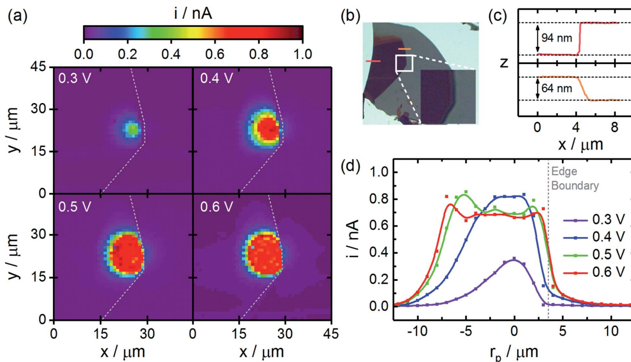
Fig. 4 CG-TC SECCM imaging of carrier transport across an individual step edge defect within an \text{n-WSe}_2 nanosheet. (a) Photocurrent images at a series of different applied potentials ( 1 \mu\text{m} resolution). (b) Optical transmission image of the \text{n-WSe}_2 nanosheet with the area imaged via SECCM and locations of the AFM height profiles indicated. (c) AFM height profiles of the \text{n-WSe}_2 nanosheet. (d) Cross-sections of the SECCM photocurrent images given in (a). SECCM data was acquired using a pipet ( d = 250 \text{ nm} , \theta_p = 8.5^\circ ) filled with an aqueous solution containing 100 \text{ mM NaI} , 10 \text{ mM I}_2 at a sweep rate of 2000 \text{ mV s}^{-1} . Imaging was carried out in the vicinity of a 633 \text{ nm} Gaussian beam with P_0 = 600 \text{ nW} and \sigma_0 = 0.73 \mu\text{m} .
