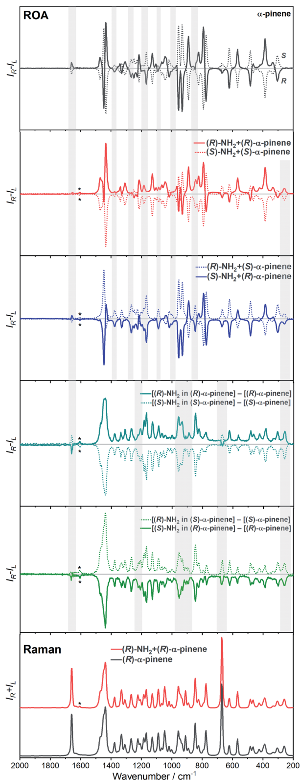
Fig. 2 The ROA spectra of (R)- and (S)- n Bu-NDI-BINAM ( R -NH 2 and S -NH 2 , respectively) dissolved in ( S )- and ( R )- \alpha -pinene. Asterisks denote the n Bu-NDI-BINAM bands. Grey belts highlight induced chirality marker bands.
