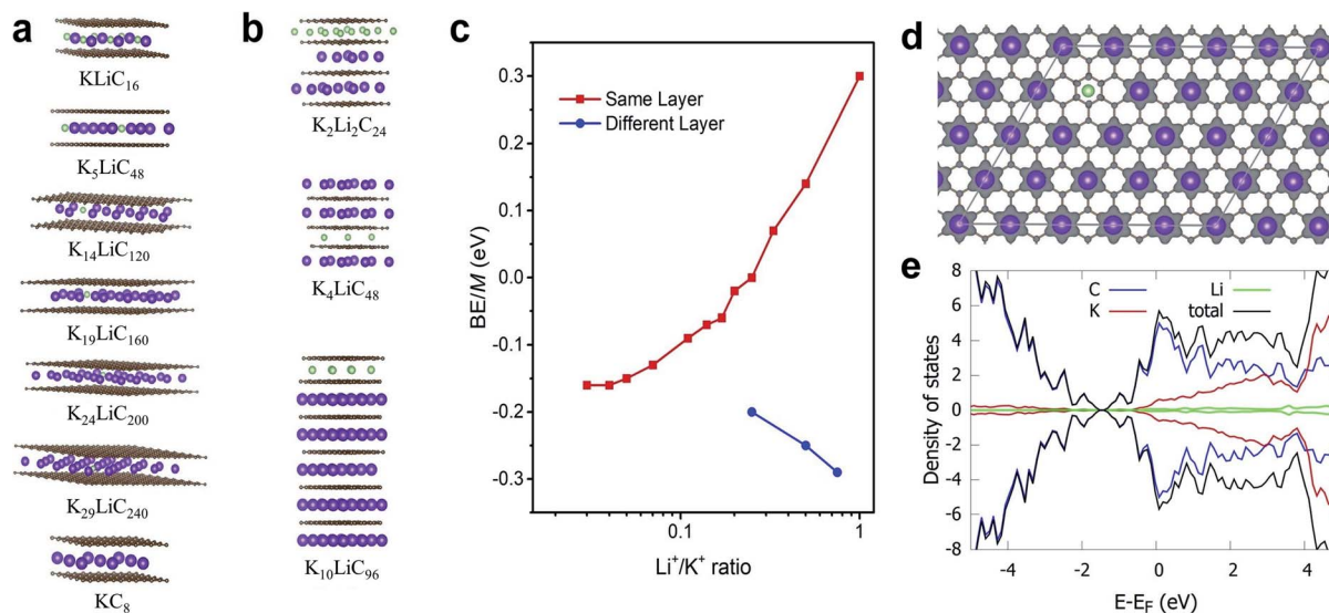
Fig. 4 Different co-intercalation configurations and corresponding metal binding energies. (a and b) Selected models showing unique Li and K co-intercalation within the same or different layers, respectively. (c) Plot of the metal binding energies corresponding to co-intercalated metals ratio of Li/K (in a logarithmic scale) within the same or different layers, respectively. (d) Charge density difference plot in a section of K_{19}LiC_{160} . Only the positive isosurface is shown for clarity. (e) Projected density of states (pDOS) in K_{29}LiC_{240} . Colouring atom scheme: Li; green, K; purple.
