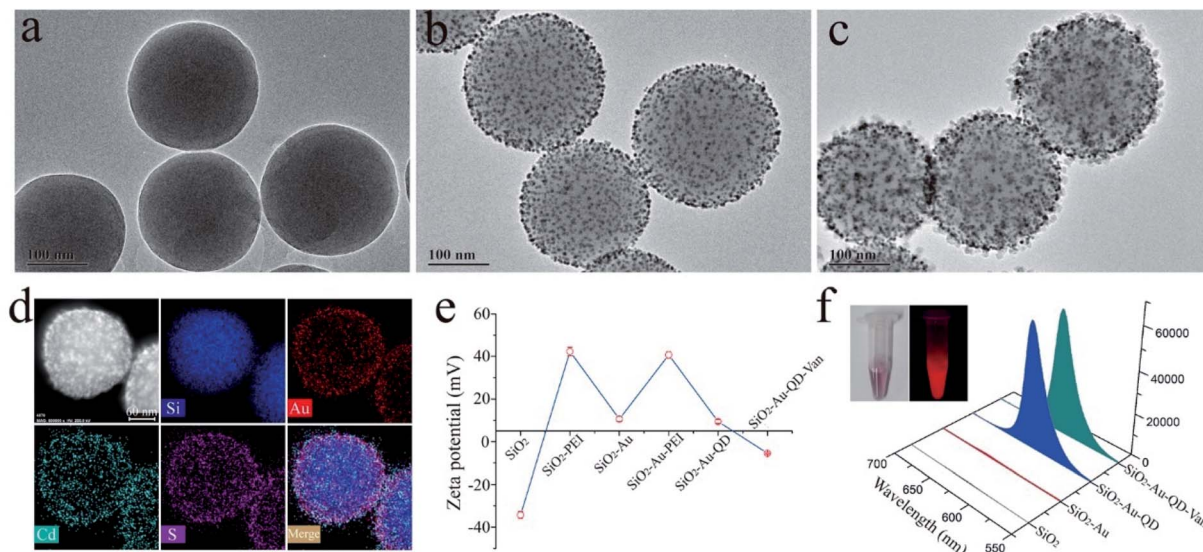
Fig. 1 Characterization of dual-signal SiO 2 -Au-QD nanotags. TEM images of (a) SiO 2 NPs, (b) SiO 2 -Au NPs, and (c) SiO 2 -Au-QD NPs. (d) EDS elemental mapping images of SiO 2 -Au-QD tags. Zeta potential results (e) and fluorescence emission spectra (f) of vancomycin-modified nanotags and their intermediate products. Inset images display the photographs of SiO 2 -Au-QD-Van tags under visible (left) and UV light (right).
