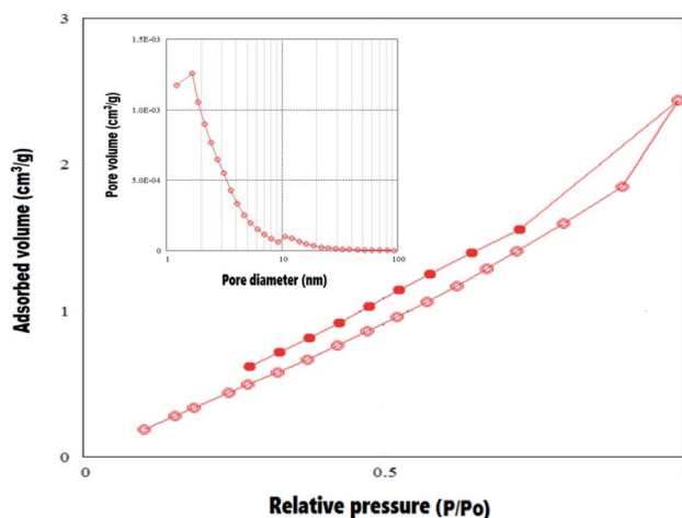
Fig. 3 Nitrogen adsorption-desorption isotherm (inset) pore size of the NFe 3 O 4 Starch-Glu-NFe 3 O 4 ED nanocomposite.
