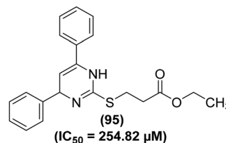
Fig. 26 Chemical structure of compound (95).
