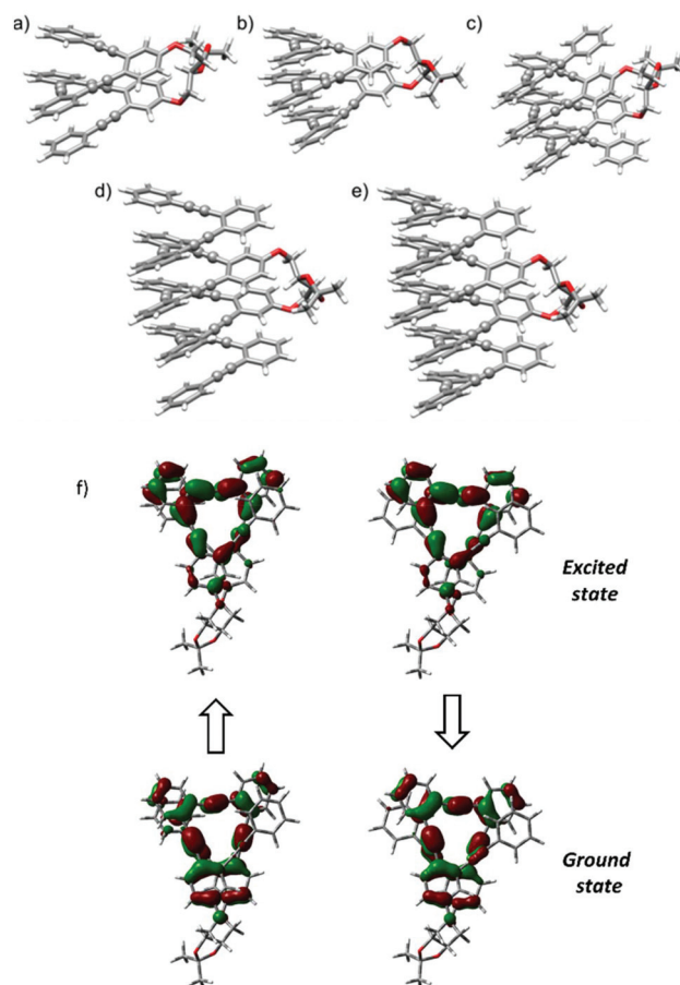
Fig. 4 Optimized DFT (B3LYP/6-31G**) structures of: (a) ( S,S,P )-2; (b) ( S,S,P )-3; (c) ( S,S,P )-4; (d) ( S,S,P )-5; (e) ( S,S,P )-6. Color coding: C, gray; O, red. H atoms have been omitted for clarity; (f) ground-excited structures and transitions for ( S,S,P )-2 in absorption (left) and emission (right).
